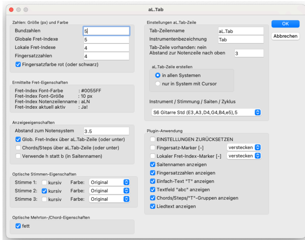
Fig. 8 Plugin-Dialogfenster
